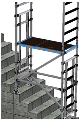
7) Fit a platform to the 3rd rung of the plain portal frame, trapdoor at the ladder frame side.
