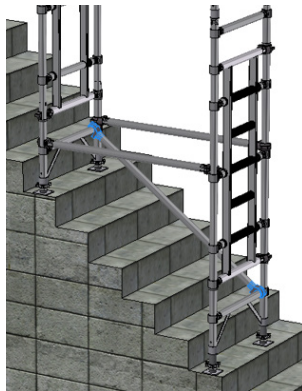
5) Fit diagonal brace from bottom rung of ladder portal frame to bottom rung of plain portal frame, on the left hand side. Then level your tower.
