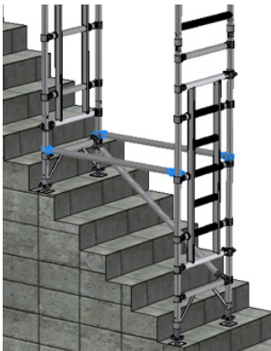
4) Position the ladder portal at the bottom of your stairs and connect the horizontal braces above the 3rd rung. Level the tower by adjusting the legs. The gates should be positioned to open outwards.
